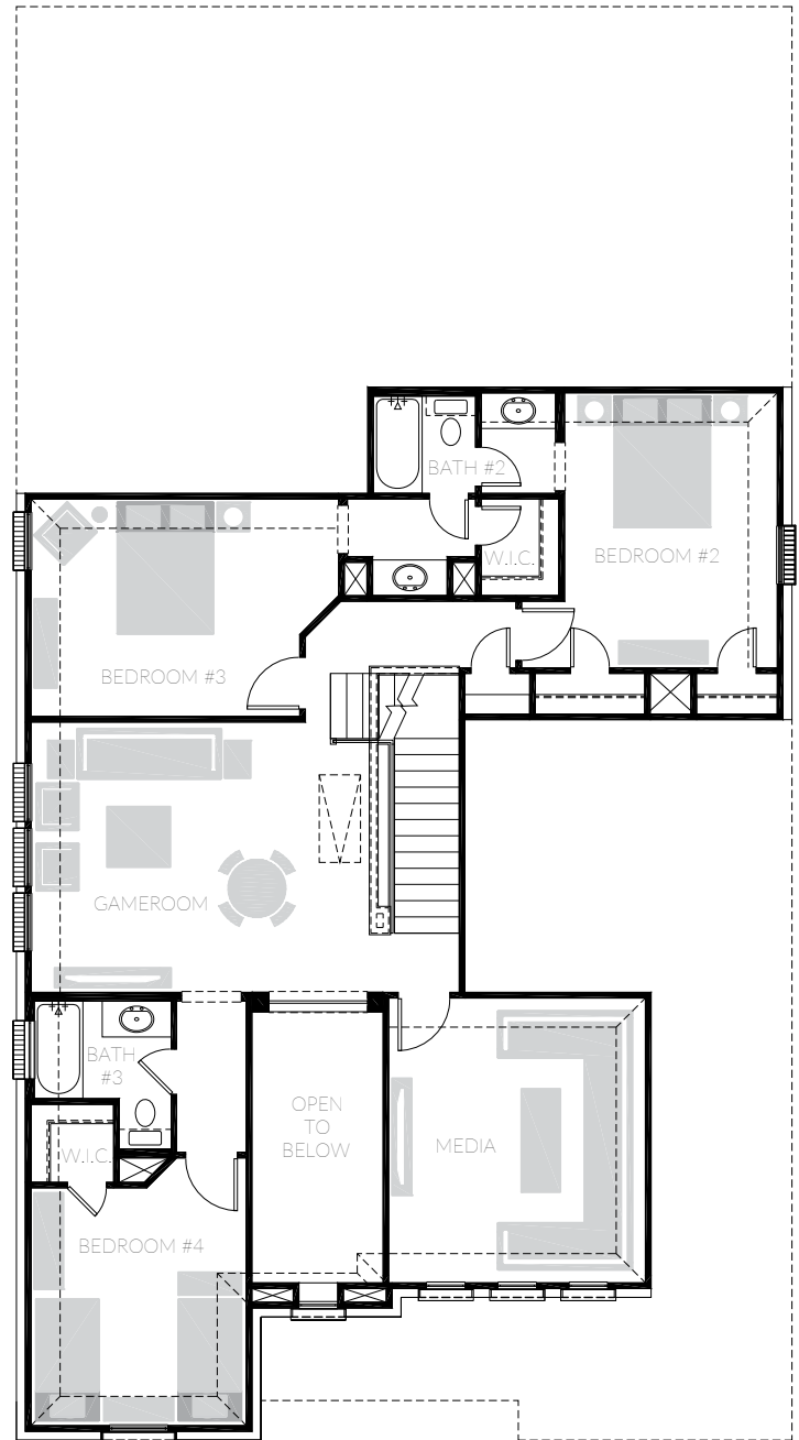
second floor
